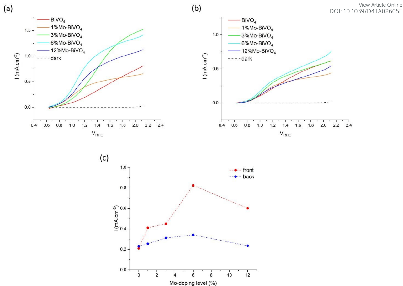
Figure 6: Current voltage (JV) curves for \text{BiVO}_4 and all Mo-doped \text{BiVO}_4 samples measured with (a) front irradiation and (b) back irradiation. (c) The photocurrent densities observed at 1.23 V_{\text{RHE}} for both front and back irradiation as a function of Mo precursor doping level (%) of \text{BiVO}_4 and all Mo-doped \text{BiVO}_4 samples. Samples were measured in 0.1 M phosphate buffer (pH = 7) using 400 nm light ( \sim 8.5 \text{ mW}\cdot\text{cm}^{-2} ).
