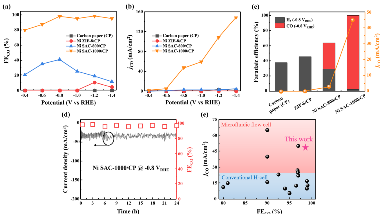
Fig. 6 (a) FE_{CO} and (b) j_{CO} at various applied potentials for Ni-based samples in CO_2 -purged 0.5 M KHCO_3 electrolytes. (c) Catalytic activities of Ni-based samples before and after pyrolysis at -0.8 V_{RHE} . (d) Stability of Ni SAC-1000 at -0.8 V_{RHE} in CO_2 -purged 0.5 M KHCO_3 . Current density (solid line) and FE_{CO} (symbol) at -0.8 V_{RHE} were plotted as a function of reaction time. (e) Summary of the catalytic activities of the Ni-based SAC for the production of CO measured with a conventional H-cell and microfluidic flow cell system.
