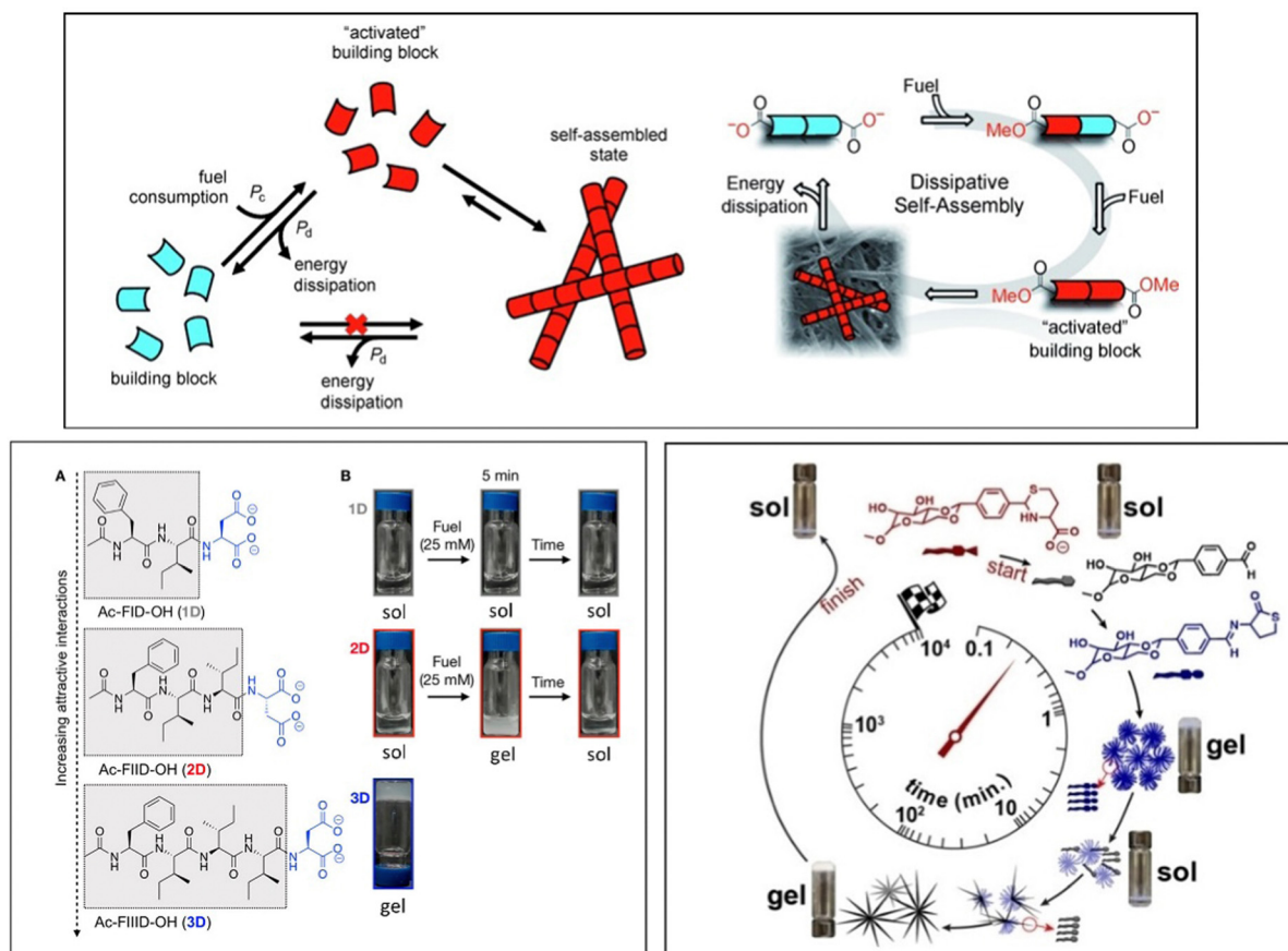
Fig. 32 Examples of fueled assembly. (top) General schematic of fueled assembly and example of fueled assembly based on esterification of dibenzoylcysteine – figure adapted and reproduced from ref. 254 with permission of Wiley-VCH, © 2010. (bottom left) Tuning a gelator for fueled assembly. If there are insufficient interactions the system remains as a sol, with too many interactions it is a gel even without fueling, and if the interactions are just right, its assembly can be transiently fueled – figure adapted and reproduced from ref. 256 with permission of the American Chemical Society, © 2020. (bottom right) System capable of transient sol–gel–sol–gel–sol assembly – figure reproduced from ref. 257 with permission of Wiley-VCH, © 2023.
