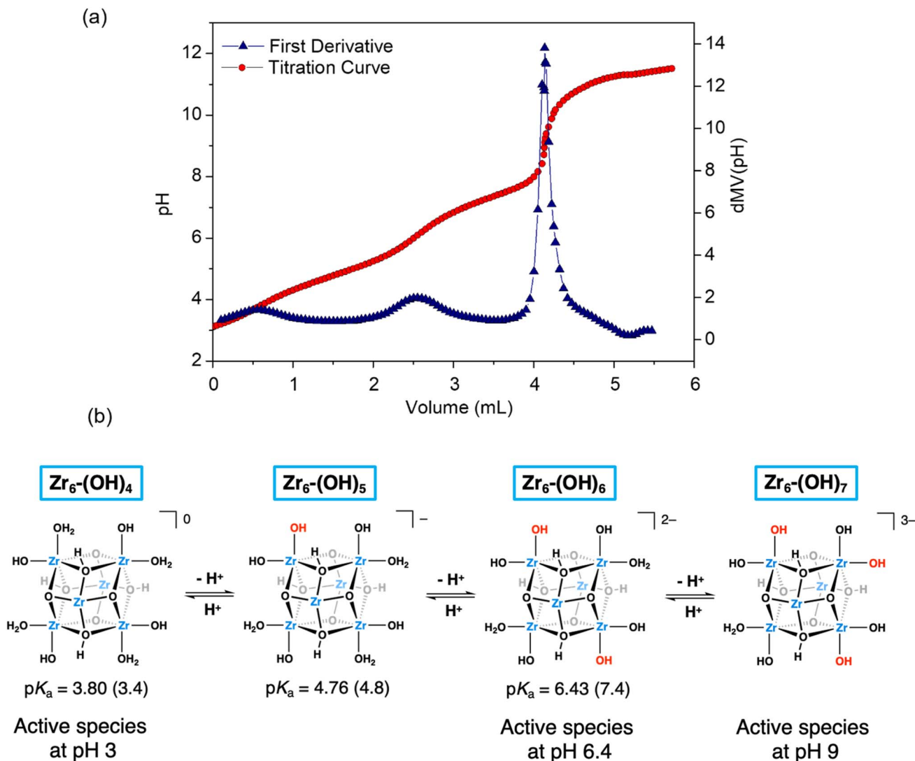
Fig. 6 (a) Zr 6 cluster titration curve (red circles) and its first derivative (blue triangles). Conditions: [Zr 6 ] = 1 × 10 -3 mol L -1 , [KCl] = 0.02 mol L -1 , water (40 mL) p H i = 3.0, p H f = 11.5, titrant KOH – 0.1 mol L -1 ; (b) proposed acid–base equilibria for Zr 6 -(OH) n species. DFT-derived assignment of the experimental p K a values are given in parentheses. Bridging acetate ligands are omitted for clarity. The stability of each species with regard to its structural isomers, which differ in the relative positions of protons, is evaluated in Scheme S3.†
