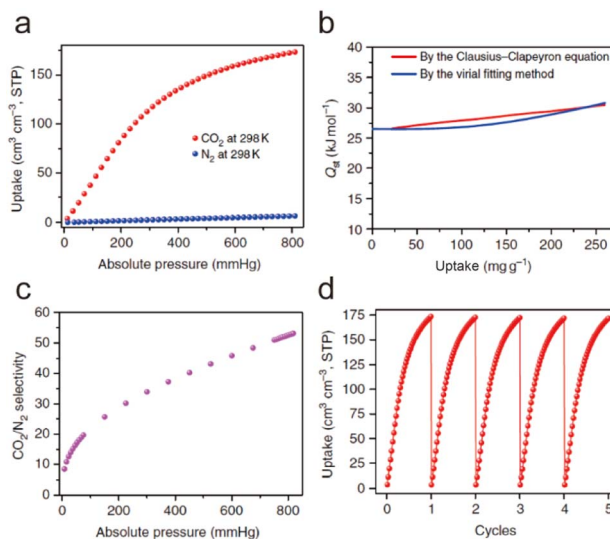
Fig. 34 (a) The \text{CO}_2 and \text{N}_2 adsorption isotherms for FJI-H14 at 298 K. (b) The isosteric heat of \text{CO}_2 adsorption ( Q_{st} ) for FJI-H14. (c) The IAST selectivity of FJI-H14 for \text{CO}_2/\text{N}_2 (15:85). (d) 5 Cycles of \text{CO}_2 adsorption for FJI-H14 at 298 K. Reproduced from ref. 136 with permission from Springer Nature, Copyright 2017.
