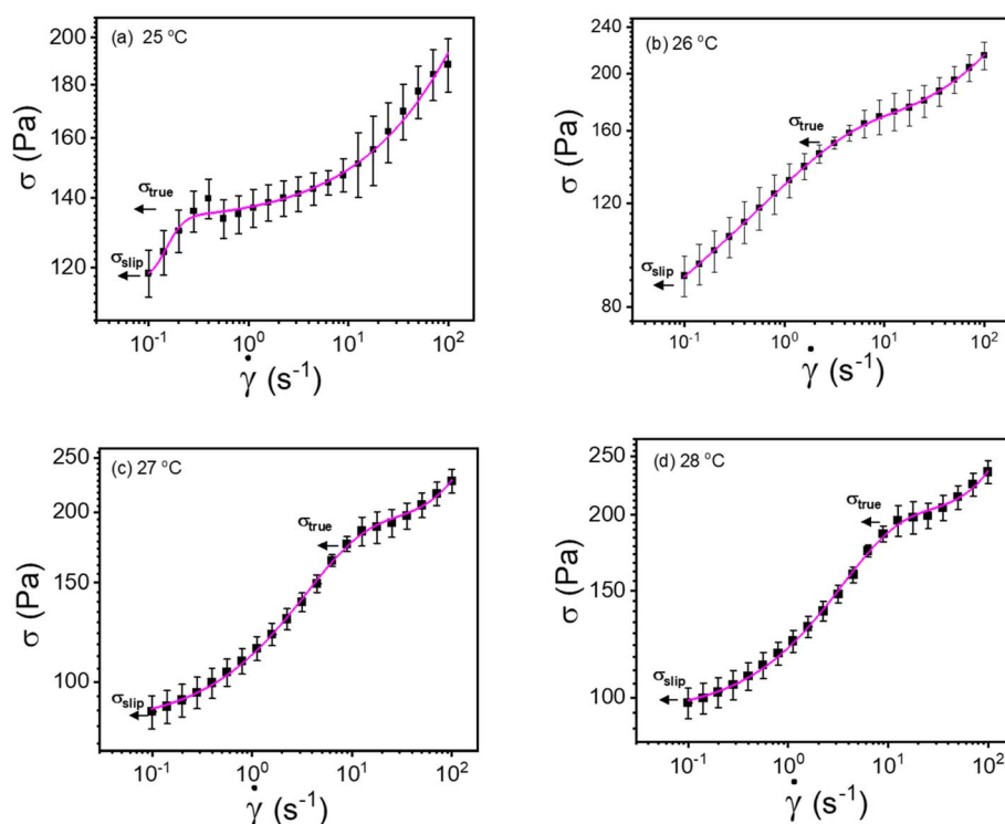
Fig. 8 (a–d) Modified Windhab model (eqn (17)) fitting of flow curves for 20% PF127 at different temperatures from 25 to 28 °C, respectively (shear rate ranges from 0.1 to 100 \text{s}^{-1} ).
