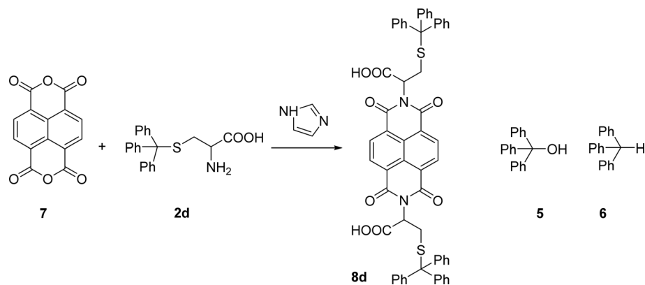
Scheme 3 Condensation of naphthalene tetracarboxylic dianhydride with cysteine- S -trityl.
