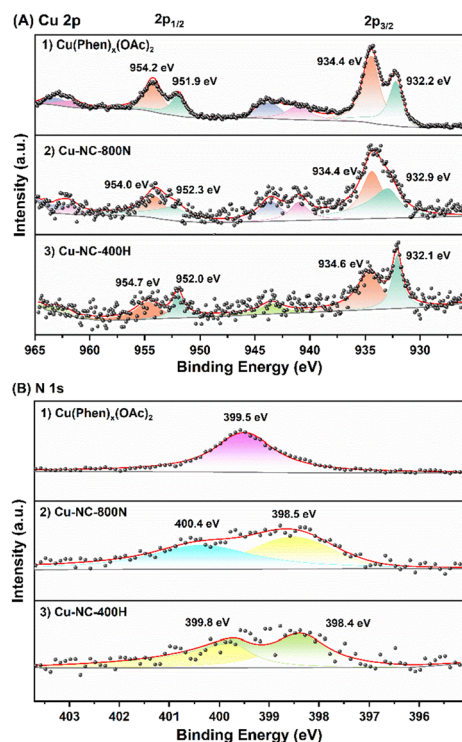
Fig. 5 The XPS of (A) Cu 2p signals: (1) \text{Cu(Phen)}_x(\text{OAc})_2 , (2) Cu-NC-800N, and (3) Cu-NC-400H samples and (B) N 1s signals: (1) \text{Cu(Phen)}_x(\text{OAc})_2 , (2) Cu-NC-800N, and (3) Cu-NC-400H samples.
