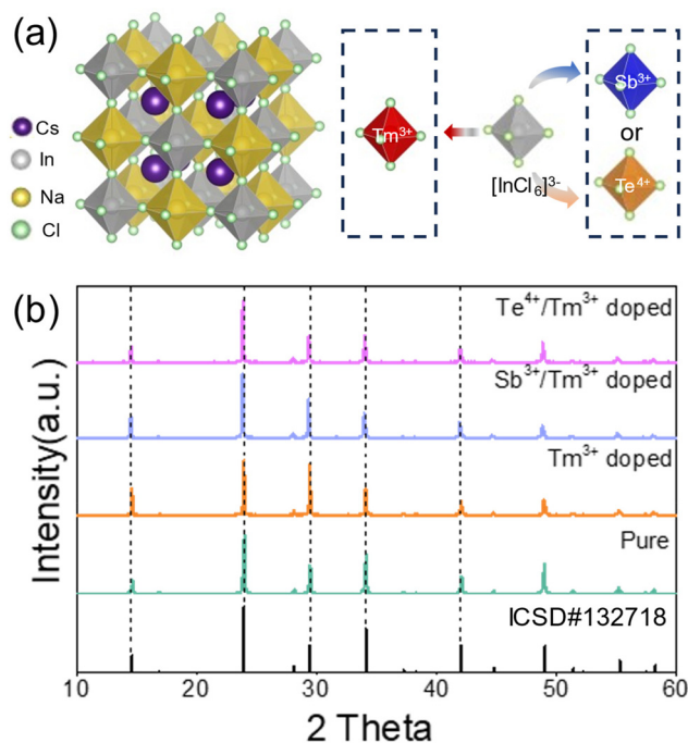
Fig. 1 (a) Structural schematic diagram of \text{Cs}_2\text{NaInCl}_6 , \text{Cs}_2\text{NaInCl}_6:\text{Sb}^{3+}/\text{Tm}^{3+} , and \text{Cs}_2\text{NaInCl}_6:\text{Te}^{4+}/\text{Tm}^{3+} double perovskites. (b) XRD patterns of pure, 5% \text{Sb}^{3+}/30\%\text{Tm}^{3+} , and 1% \text{Te}^{4+}/30\%\text{Tm}^{3+} doped \text{Cs}_2\text{NaInCl}_6 .
