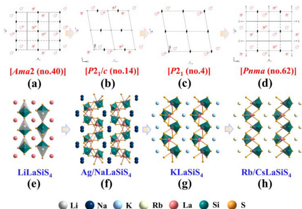
Fig. 3 Structural fluctuations in A^I\text{LaSi}_4 ( A^I = \text{Li, Ag, Na, K, Rb, Cs} ): (a–d) symmetry changes from Ama2 (LiLaSi 4 ), P2_1/c (AgLaSi 4 /NaLaSi 4 ), and P2_1 (KLaSi 4 ) to Pnma (RbLaSi 4 and CsLaSi 4 ); (e–h) the crystal structures of LiLaSi 4 (e), Ag/NaLaSi 4 (f), KLaSi 4 (g), and Rb/CsLaSi 4 (h).
