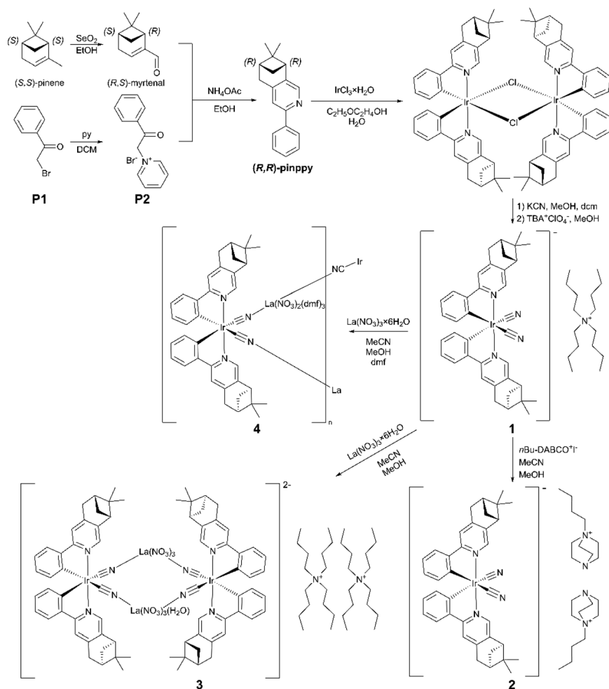
Scheme 1 Reported synthetic route for an enantiopure (R,R) -pinppy ligand starting from (S,S) -pinene and 2'-bromoacetophenone (P1), and further syntheses of compounds 1–4 which are based on chiral dicyanidoiridate(III) complexes bearing the deprotonated form of (R,R) -pinppy. In all cases, the chirality at the ligand is of the (R,R) -type, whereas the detected diastereoisomers related to the chirality at the metal differ, i.e., the \Delta -isomers are present for 1 and 2, while the \Lambda -isomers are observed in 3 and 4. They are properly visualized in this scheme (see the text for details).
