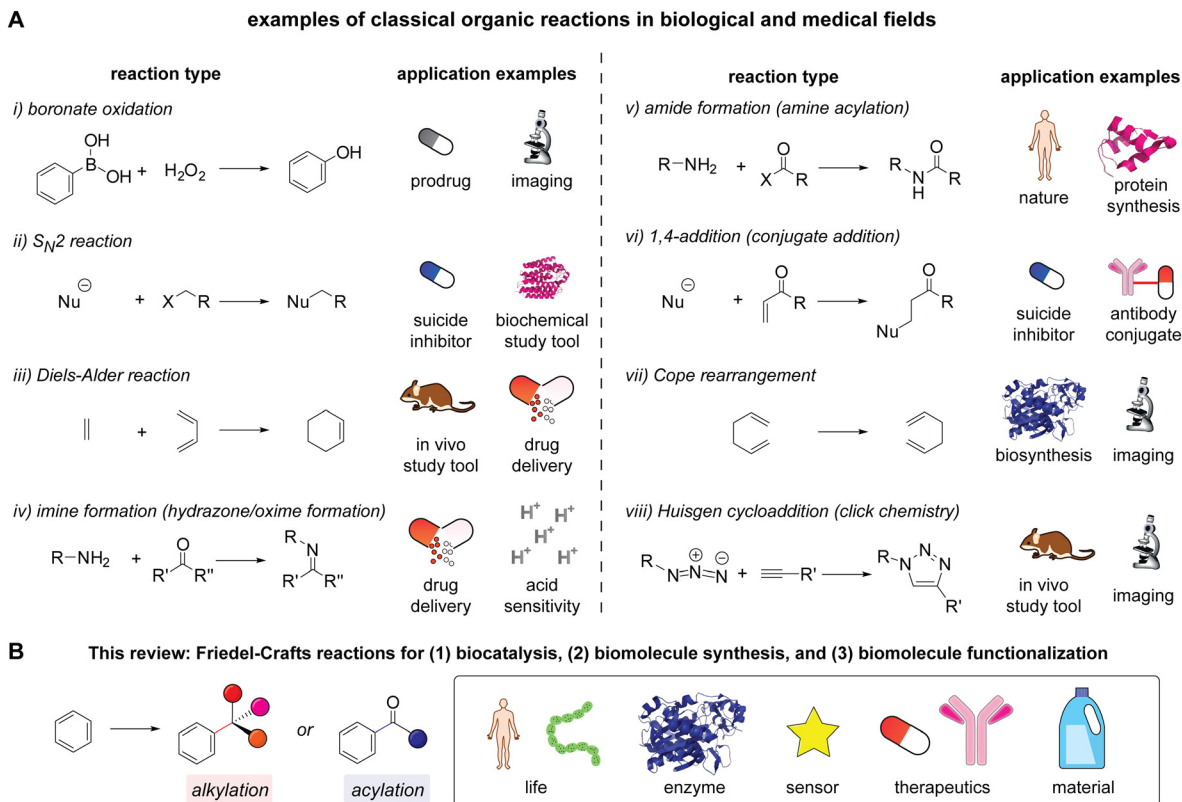
Scheme 1 Classical organic reactions in biological and medical fields. (A) Examples of the classical organic reactions including: (i) boronate oxidation, 1,2 (ii) S_N2 reactions with fluoro- and iodoacetamide, 3,4 (iii) Diels–Alder reactions for bioorthogonal chemistry, 5,6 (iv) imine and relevant C=N bond formation such as hydrazone and oxime, 7,8 (v) amide formation such as protein expression and native chemical ligation, 9,10 (vi) 1,4-addition to a carbonyl group such as acrylamide and maleimide, 11,12 (vii) Cope rearrangement, 27–29 and (viii) Huisgen cycloaddition or azide–alkyne cycloaddition. 18,30 The organization of the reactions is based on the appearance in an Organic Chemistry textbook (Marc Loudon and Jim Parise, sixth edition). (B) Friedel–Crafts alkylation and acylation for biomolecular chemistry as a theme of this review.
