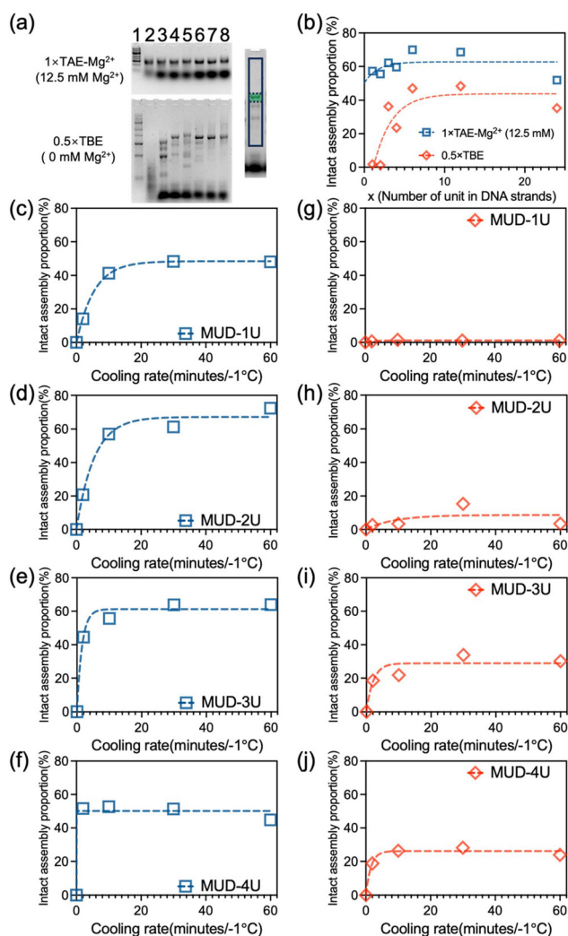
Fig. 4 (a) Images of a series of MUD- x U samples under agarose-gel electrophoresis with 1× TAE- Mg^{2+} ( Mg^{2+} = 12.5 mM) buffer (upper-left panel) and 0.5× TBE buffer ( Mg^{2+} = 0 mM) (lower-left panel). All MUD- x U samples were assembled with 20 mM Mg^{2+} in the buffer. Lanes 1, 2, 3, 4, 5, 6, 7, and 8: double-stranded DNA ladder (GeneRuler Express DNA Ladder, Thermo Fisher Scientific), MUD-1U, MUD-2U, MUD-3U, MUD-4U, MUD-6U, MUD-12U, and MUD-24U, respectively. Right panel: areas of intact assembly and total assembly products used for calculating the proportion of intact assemblies were marked by the green mask and black box, respectively. (b) Analyses of intact proportions of a series of MUD- x U samples under agarose-gel electrophoresis with 1× TAE- Mg^{2+} buffer ( Mg^{2+} = 12.5 mM, marked by blue boxes) and 0.5× TBE buffer ( Mg^{2+} = 0 mM, marked by red diamonds). The intact assembly proportions of (c and g) MUD-1U, (d and h) MUD-2U, (e and i) MUD-3U, and (f and j) MUD-4U with different cooling rates under agarose-gel electrophoresis containing 12.5 mM Mg^{2+} (marked in blue boxes) and 0 mM Mg^{2+} (marked in red diamonds). The one-phase decay-fitting curves corresponding to the sample data in the same color are presented in (b)–(j).
