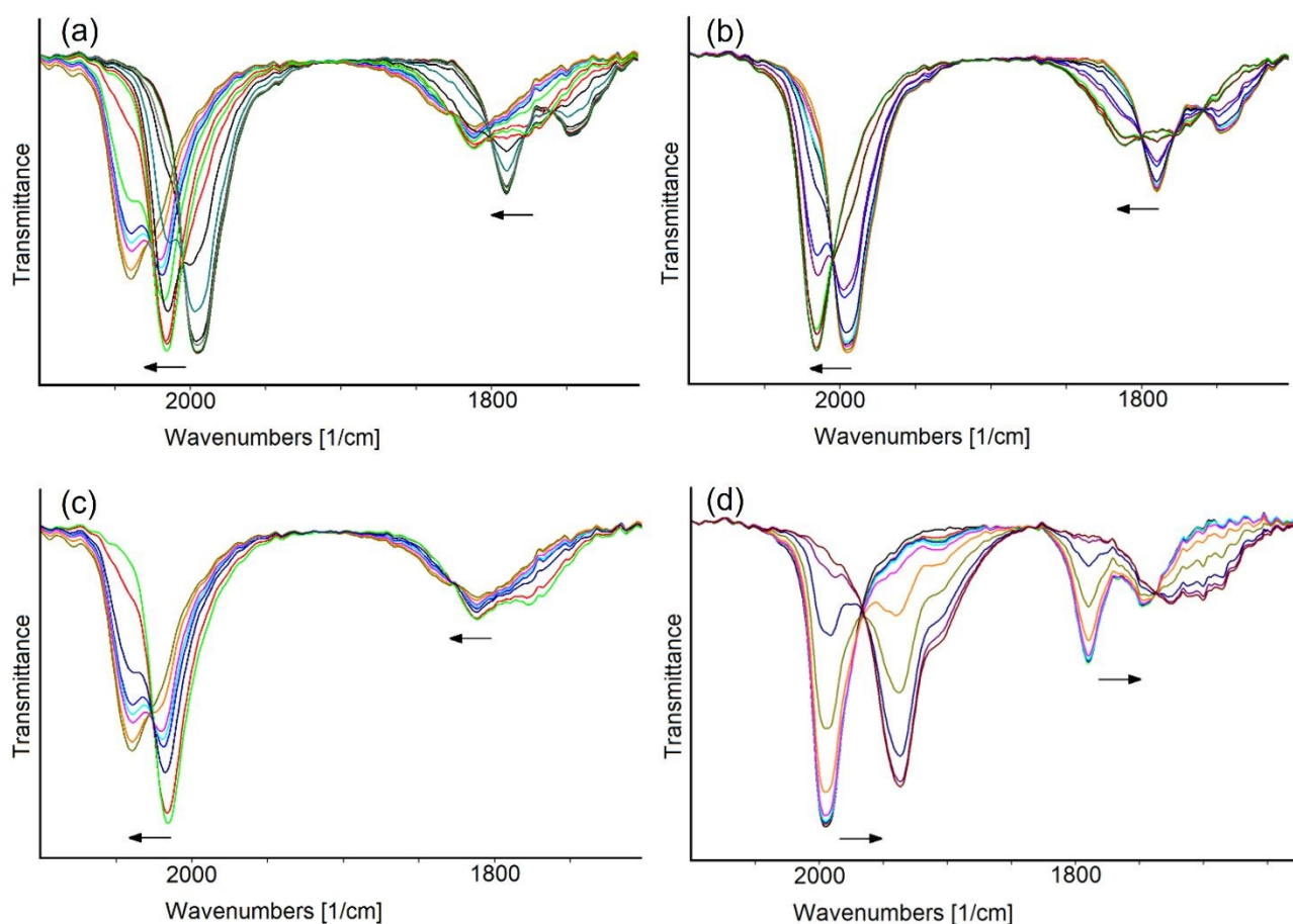
Figure 5. IR spectral changes of a \text{CH}_3\text{CN} solution of [\text{Rh}_{12}\text{In}(\text{CO})_{28}]^{3-} recorded every 60 sec in an OTTLE cell during the progressive (scan rate 1\text{ mV sec}^{-1} ) increase of the potential from -0.40 to +0.50 V (a); progressive increase of the potential from -0.40 to +0.10 V (b); progressive increase of the potential from +0.10 to +0.50 V (c); progressive decrease of the potential from -0.40 to -1.85 V (d). The solvent and supporting electrolyte absorptions have been subtracted.
