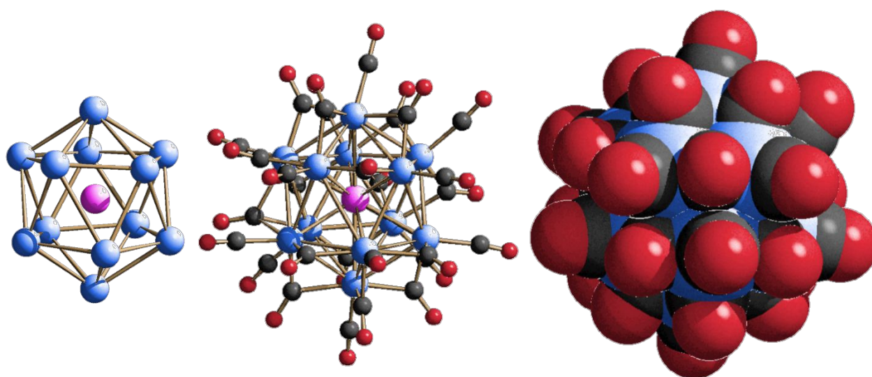
Figure 1. Metal skeleton (left), molecular structure (centre) and space-filling model (right) of [\text{Rh}_{12}\text{In}(\text{CO})_{28}]^{3-} ( 1 ). Rh is depicted in blue, In in magenta, C in grey, and O in red.
