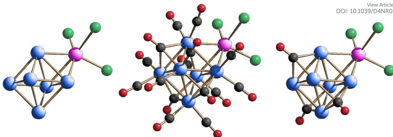
Figure 2. Metal skeleton (left), molecular structure (centre) and face-bridging ligand arrangement (right) of [\text{Rh}_6(\text{CO})_{15}\text{InCl}_3]^{2-} ( 2 ). Rh is depicted in blue, In in magenta, Cl in green, C in grey, and O in red.
