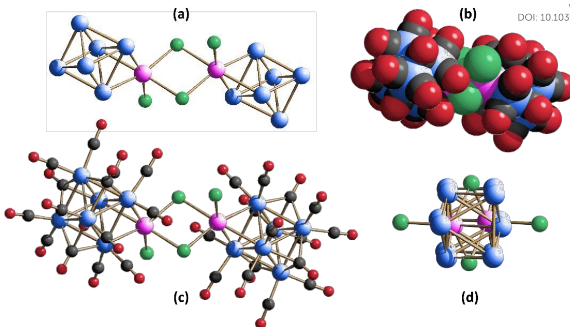
Figure 3. Metal skeleton (a), space-filling model (b), molecular structure (c) and eclipsed view of the two octahedral \text{Rh}_6 moieties (d) of [\{\text{Rh}_6(\text{CO})_{15}\text{InCl}_2\}_2]^{2-} ( 3 ). Rh is depicted in blue, In in magenta, Cl in green, C in grey, and O in red.
