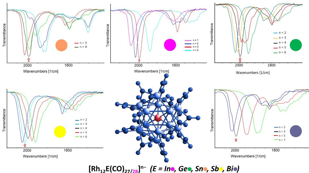
Figure 8. Multivalence behaviour of the [\text{Rh}_{12}\text{E}(\text{CO})_{27/28}]^{n-} family of clusters ( n = 3 when E = In, Sb, Bi; n = 4 when E = Ge, Sn) family of clusters as obtained by spectroelectrochemical experiments. 27
