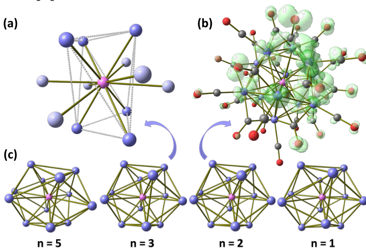
Figure 7. DFT-optimized \{\text{Rh}_{12}\text{In}\} core of 1 . The Rh atoms are connected to the central In (magenta) to highlight the outcomes of the AIM analysis. The Rh atoms involved in the strongest interactions are blue coloured, while the others are light blue coloured (a). DFT-optimized structure of [\text{Rh}_{12}\text{In}(\text{CO})_{28}]^{2-} with spin density surface (isovalue = 0.002 a.u., green tones) (b). \{\text{Rh}_{12}\text{In}\} cores of the DFT-optimized structures of [\text{Rh}_{12}\text{In}(\text{CO})_{28}]^{n-} ( n = 5, 3, 2, 1 ) (c). Colour map: Rh, blue; In, magenta; C, grey; O, red.
