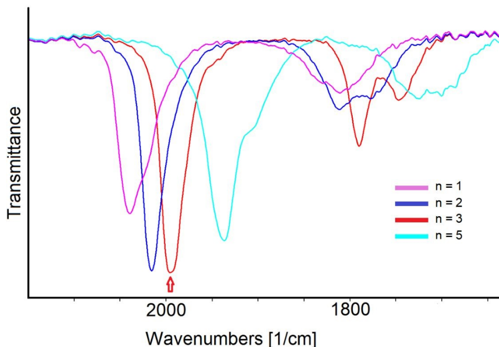
Figure 6. Selected infrared spectra of [\text{Rh}_{12}\text{In}(\text{CO})_{28}]^{n-} as a function of the cluster charge n in \text{CH}_3\text{CN} containing 0.1 \text{ mol dm}^{-3} [\text{N}^n\text{Bu}_4][\text{PF}_6] . The absorptions of the solvent and supporting electrolyte have been subtracted. The red arrow indicates the initial spectrum.
