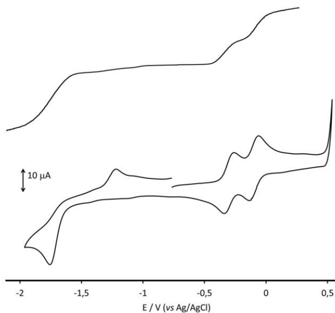
Figure 4. Cyclic (bottom) and hydrodynamic (top) voltammetric responses recorded at a GC electrode in a \text{CH}_3\text{CN} solution of [\text{Rh}_{12}\text{In}(\text{CO})_{28}]^{3-} under \text{CO} atmosphere. [\text{N}^n\text{Bu}_4][\text{PF}_6] ( 0.1 \text{ mol dm}^{-3} ) as the supporting electrolyte. Scan rate = 0.1 \text{ V s}^{-1} .
