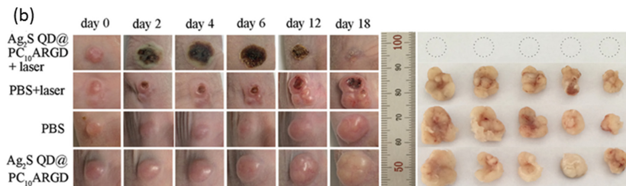
Fig. 8 (a) A general scheme for the preparation of nanogels for fluorescence and PA imaging-guided photothermal therapy. (b) The effect of PTT on tumor-bearing mice (left) and extracted tumors (right). Reproduced with permission. 138 Copyright 2018, The Royal Society of Chemistry.
