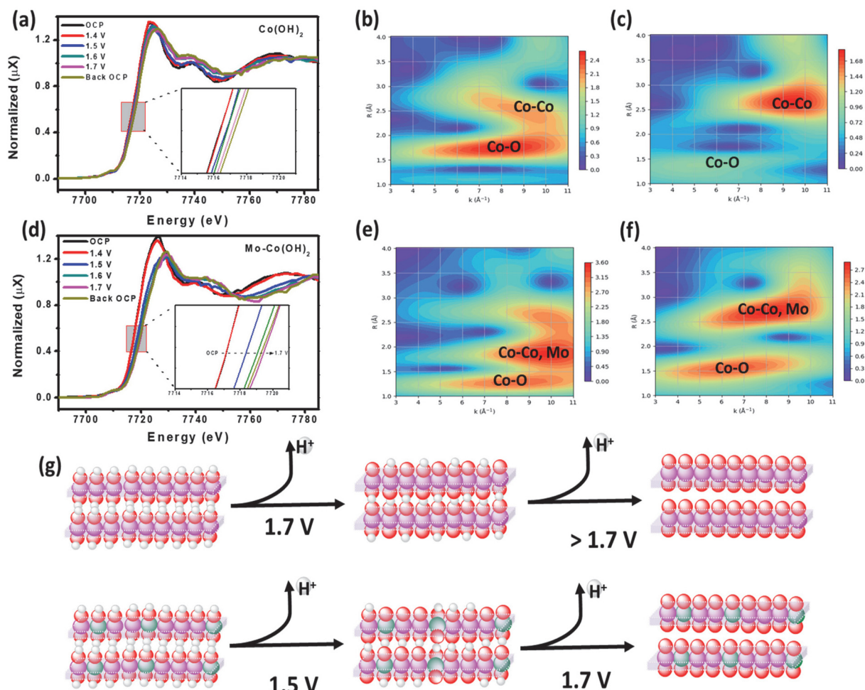
Fig. 4 (a) Operando XAFS Co K-edge absorption spectra of Co(OH) 2 , wavelet transformation of the k 2 -weighted Co K-edge absorption EXAFS signals of Co(OH) 2 at (b) 1.4 V and (c) 1.7 V, (d) operando XAFS Co K-edge absorption spectra of Mo-Co(OH) 2 , (e) wavelet transforms of the k 2 -weighted Co K-edge absorption EXAFS signals of Mo-Co(OH) 2 at (e) 1.4 V and (f) 1.7 V. (g) Schematic of the oxidation process of Co(OH) 2 to CoOOH during the OER: O (red), H (white), Co (purple), and Mo (green).
