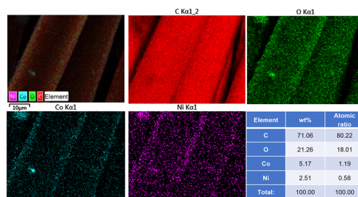
Fig. 5 EDS mapping and the atomic ratio of elements in \text{CoNi}_{0.5}\text{-MOF/CC} .
