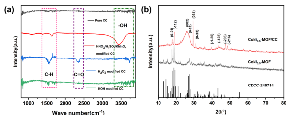
Fig. 3 (a) FT-IR spectra of carbon cloth under different treatments; (b) XRD patterns of \text{CoNi}_{0.5}\text{-MOF} and \text{CoNi}_{0.5}\text{-MOF/CC} .
