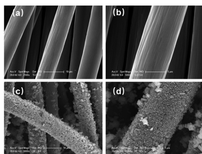
Fig. 4 SEM images of (a and b) \text{H}_2\text{O}_2 -pretreated CC substrate and (c and d) \text{CoNi}_{0.5}\text{-MOF/CC} at different magnifications.
