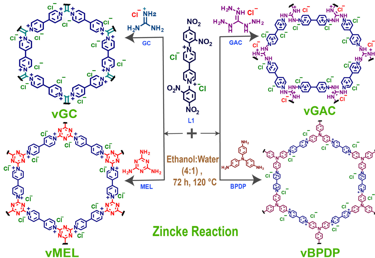
Fig. 1 Schematic representation of the synthesis of vCONs (vGC, vGAC, vMEL, and vBPDP) by the Zincke reaction of L1 with the respective triamines (GC, GAC, MEL, and BPDP).
