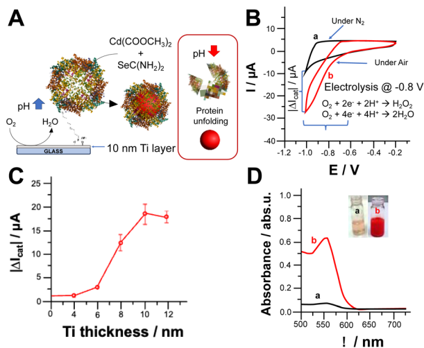
Fig. 1 (A) Scheme of electrochemically triggered local pH change; (B) cyclic voltammograms recorded with the Ti modified electrode with ferritin (1 \text{cm}^2 geometrical area) with the absence (a) and presence of \text{O}_2 (in equilibrium with air). Potential scan rate, 5 \text{mV s}^{-1} . Background electrolyte: \text{NH}_3/\text{acetate} buffer (3 mM, pH 6.5 containing 0.1 M \text{Na}_2\text{SO}_4 ); (C) catalytic current measurements at -0.8 V vs. Ag/AgCl correlated to Ti thickness; (D) UV-Vis spectra of reaction media after applying -0.8 V vs. Ag/AgCl for 30 min in the absence (a) and presence of \text{O}_2 (in equilibrium with air) – insets: photo of reaction media before (a) and after (b) electrochemically triggered CdSe NPs synthesis.
