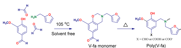
Scheme 1 Synthesis of the V-fa monomer and polymerization of poly(V-fa).
