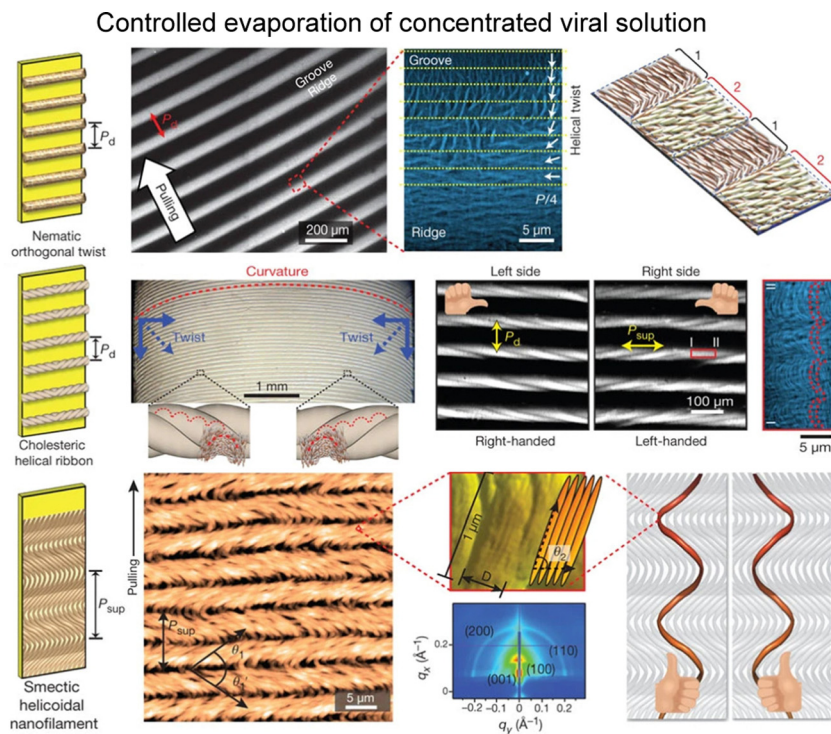
Fig. 13 Filamentous bacteriophage self-assembly. Film morphologies of M13 bacteriophage films; nematic orthogonal twist (first row), cholesteric helical ribbon (second row), and smectic helicoidal nanofilament (third row). The figure is reproduced from ref. 120 with permission from Springer Nature, copyright 2011.
