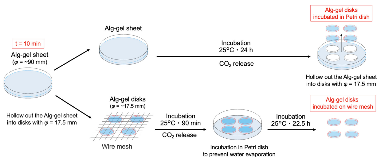
Fig. 5 Schematic preparation of the Alg-gel disks incubated in the Petri dish and on the wire mesh for mechanical evaluations. t = 0 refers to the time as carbonated water was added.
