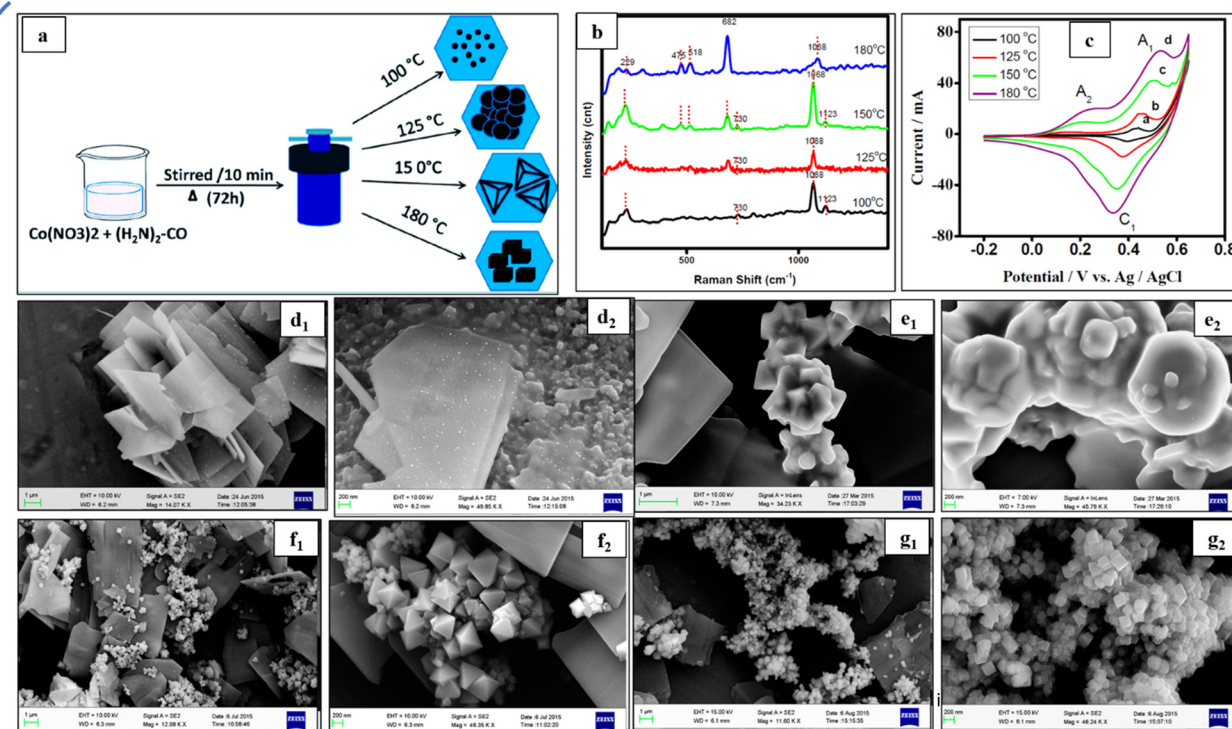
Fig. 12 (a) Schematic illustration of the synthesis process and the resulting structures. (b) Raman shift and (c) CV of all synthesized samples at 50 mV s -1 . Low and high magnification images of the \text{Co}_3\text{O}_4 electrode obtained at (d 1 ) and (d 2 ) 100 °C, (e 1 ) and (e 2 ) 125 °C, (f 1 ) and (f 2 ) 150 °C, and (g 1 ) and (g 2 ) 180 °C. Reproduced with permission from ref. 161. Copyright 2017 MDPI publications.
