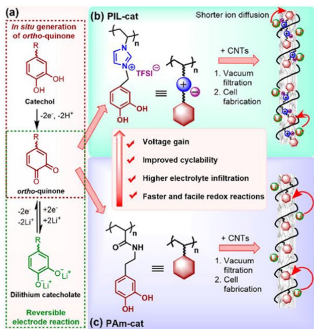
Fig. 32 Construction of catechol-based PIL/CNTs buckypaper for LIBs. (a) ortho -Quinone/di-lithium catecholate redox reaction. (b and c) Enhancement in the electrochemical performance of cationic PIL-cat (b) compared to its neutral counterpart PAm-cat (c). Reproduced from ref. 212 with permission from ACS, Copyright [2018].
