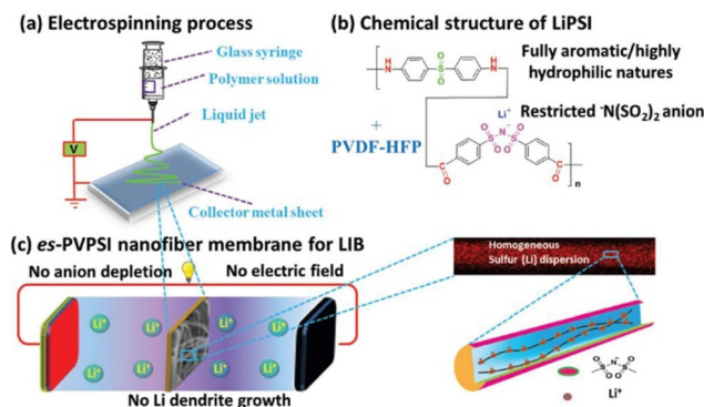
Fig. 33 Schematic illustration of the fabrication (a), composition (b), and operation (c) of the es-PVPSI nanofiber-based membrane acting as single-ion conducting polymer electrolyte in LIBs. Reproduced from ref. 213 with permission from Wiley-VCH, Copyright [2019].
