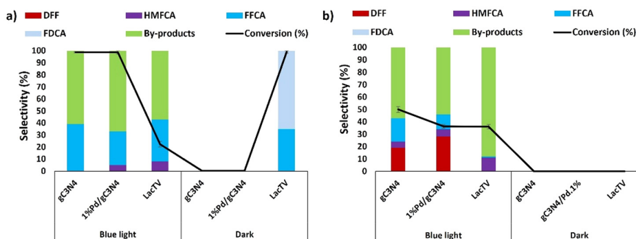
Fig. 7 Oxidation of HMF by LacTV, gC_3N_4 , and 1%Pd/ gC_3N_4 in (a) TEMPO-mediated and (b) without TEMPO, in the presence and absence of blue light. Compounds: 2,5-furandicarboxaldehyde (DFF); 5-formyl-2-furoic acid (FFCA); 2,5-furandicarboxylic acid (FDCA) and 5-hydroxymethyl-2-furancarboxylic acid (HMFCFA); catalyst: gC_3N_4 (graphitic carbon nitride), 1%Pd/ gC_3N_4 (graphitic carbon nitride with 1% palladium) and LacTV (free laccase from Trametes versicolor ). Conditions: HMF (75 mM), TEMPO (0.3 equivalents), chemical catalyst (10 mg), LacTV (5U), citrate buffer (pH 6.0, 75 mM), reaction time (24 h), 400 rpm at 30 °C (dark) and blue light (460 nm).
