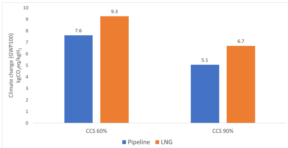
Fig. 10 Blue hydrogen CO 2 capture rate of 60% vs. 90%.
