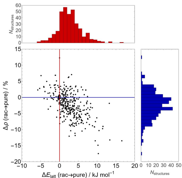
Fig. 9 The difference in lattice energy ( \Delta E_{latt} , top red histogram) and relative density ( \Delta\rho , right blue histogram) between the energy minimum in Sohncke (enantiopure) space groups and that in racemic space groups, for all molecules in our set containing at least one chiral centre. The scatter plot (center) displays the relationship between these values for each comparison (red and blue lines indicate the origin, i.e. no change in either quantity).
