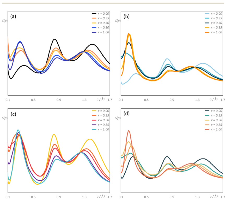
Fig. 9 Total structure factor functions, S(q) : (a) [C_8MIM]_{1-x}[C_8MIM-F_{13}]_x[Tf_2N] ; (b) [C_8MIM]_{1-x}[C_{10}MIM-F_{17}]_x[Tf_2N] ; (c) [C_{10}MIM]_{1-x}[C_8MIM-F_{13}]_x[Tf_2N] ; (d) [C_{10}MIM]_{1-x}[C_{10}MIM-F_{17}]_x[Tf_2N] mixtures. Data for (a) at 300 K and for (b) to (c) at 333 K.
