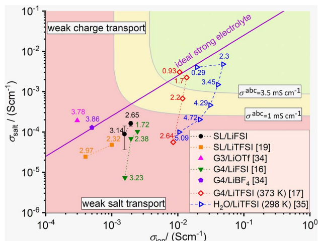
Fig. 8 Plot of the salt transport coefficient \sigma_{\text{salt}} vs. the ionic conductivity \sigma_{\text{ion}} for classifying different electrolytes. 16,17,19,34,35 The data points with filled symbols result from experiments at 303 K, while the data points with open symbols result from MD simulations at the given temperature. The straight line in magenta represents an ideal strong electrolyte without any ion correlations. Electrolytes above this line show weak charge transport properties, while electrolytes below this line show weak salt transport properties. Two iso- \sigma^{\text{abc}} lines with \sigma^{\text{abc}} values of 3.5 \text{ mS cm}^{-1} and 1 \text{ mS cm}^{-1} , respectively, are sketched for assessing the \text{Li}^+ transport in the electrolyte under anion-blocking conditions in a lithium-ion battery. The numbers next to the data points give the salt concentration of the electrolytes in \text{mol l}^{-1} .
