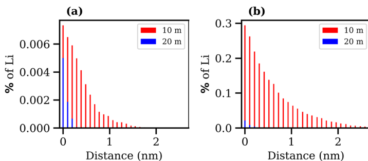
Fig. 10 Bar charts presenting the distance travelled by Li + ions that migrate from (a) the LiTFSI phase to the LiCl phase, for the 10 molal biphasic system (red) and 20 molal biphasic system (blue) and (b) the LiCl phase into the LiTFSI phase over the final 10 ns of the trajectory. The y-axis shows the percentage of Li + ions that move relative to the total number of Li + ions in the phase they move from. The x-axis represents the z-depth of penetration that those Li + move into the second phase, measured from the Gibbs dividing surface.
