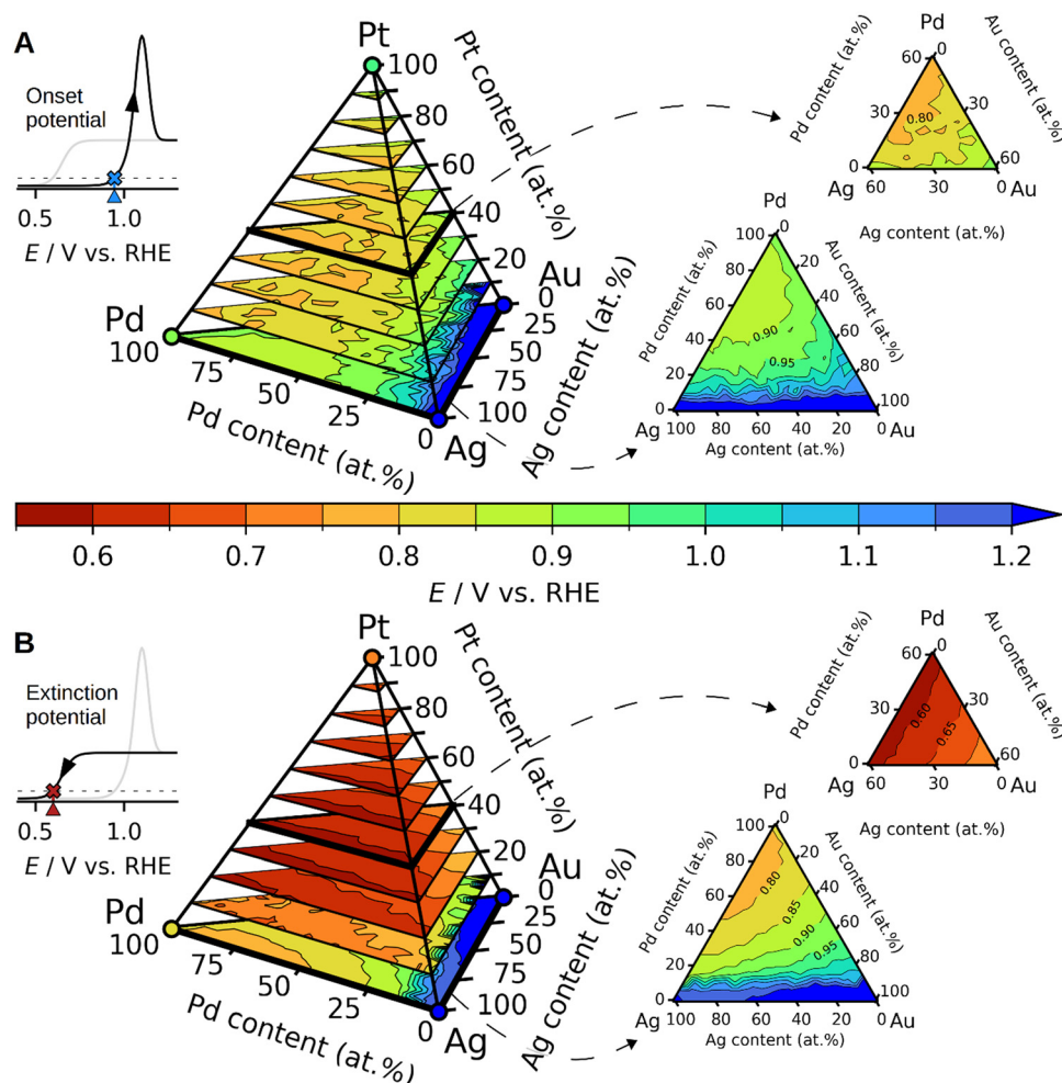
Fig. 6 Simulated CO oxidation potentials as a function of the composition in the quaternary AgAuPdPt composition space. (A) Onset potentials simulated as the potential at which ^*\text{OH} can adsorb to a surface equilibrated with ^*\text{CO} . (B) Extinction potentials, i.e. where the CO oxidation ceases, simulated as the potential at which ^*\text{OH} can adsorb to a surface without adsorbed ^*\text{CO} . Both A and B are slices of the quaternary composition space highlighted corresponding to constant Pt concentrations of 0 and 40 at%.
