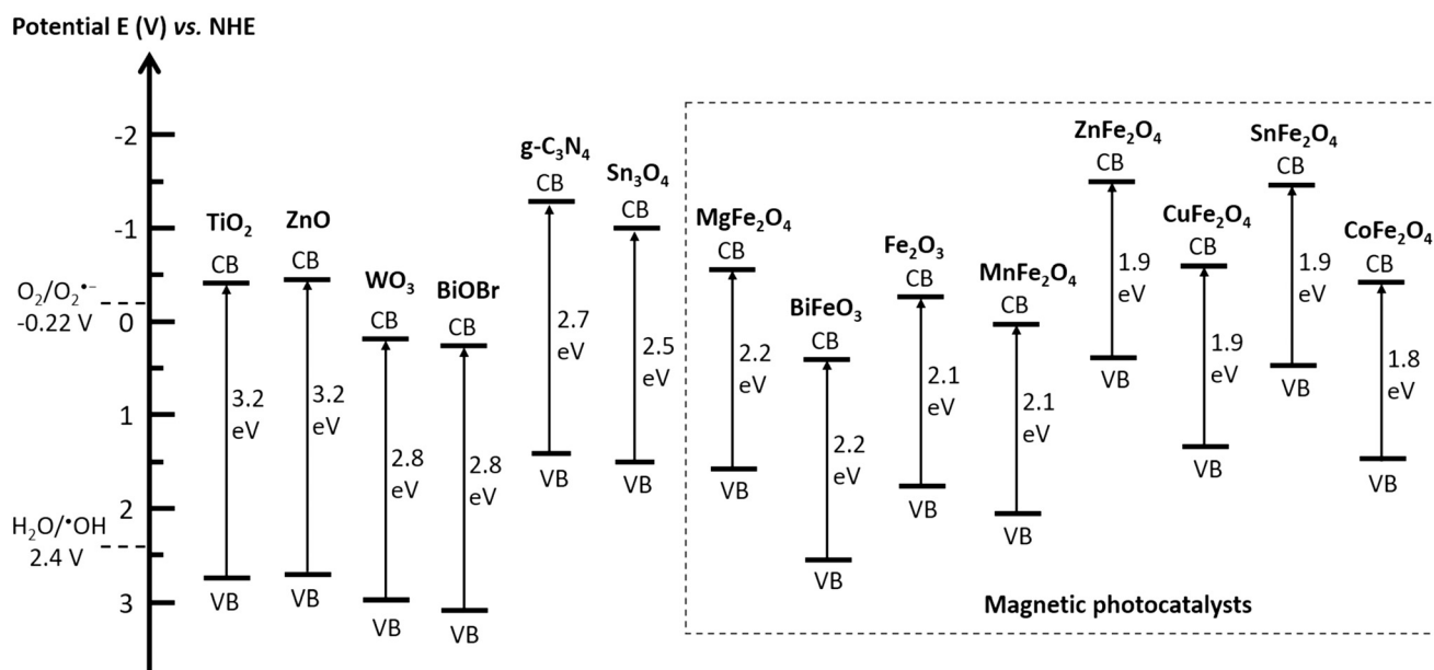
Fig. 2 Band gap energies of the involved photocatalysts in the reviewed MRNPCs and redox potentials of oxygen reduction and water oxidation to produce reactive oxygen species at pH 7.
