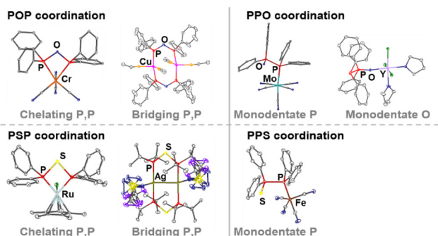
Fig. 5 Selected examples of XPX- and PPX-based coordination compounds. 4,8,9,11,14 Hard metals result in oxygen coordination and soft metals in phosphorus coordination. An equilibrium shift of the PPX to the XPX tautomer can occur, which results in the formation of coordination-stabilised tautomers, such as seen with the dinuclear copper complex and the mononuclear Ru- and Cr-based chelate complexes.
