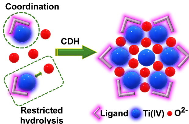
Fig. 3 Coordination-delayed-hydrolysis (CDH) method.
