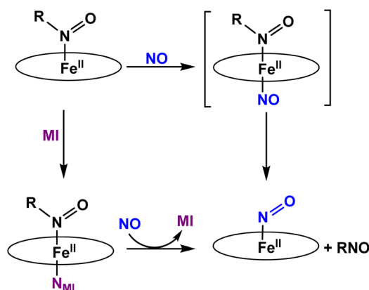
Scheme 3 Summary of the reactivity observed for five- and six-coordinate ferrous heme-RNO (R = IPr and PhNO) complexes with the \text{TPP}^{2-} ligand with NO.
