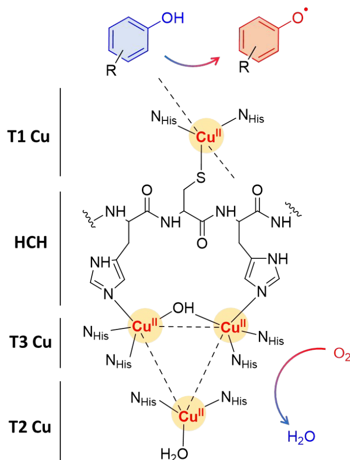
Figure 1. Schematic representation of the laccase catalytic site processing a phenolic compound. Type-1 Copper site (T1 Cu) located at the surface of the substrate binding pocket with one copper atom coordinating two histidine residues and one cysteine residue. In addition, T1 Cu has two weakly coordinating residues in the axial position that vary depending on the source of the enzyme (typically Phe or Leu for high-potential fungal laccases or Met for low-potential bacterial laccases).
