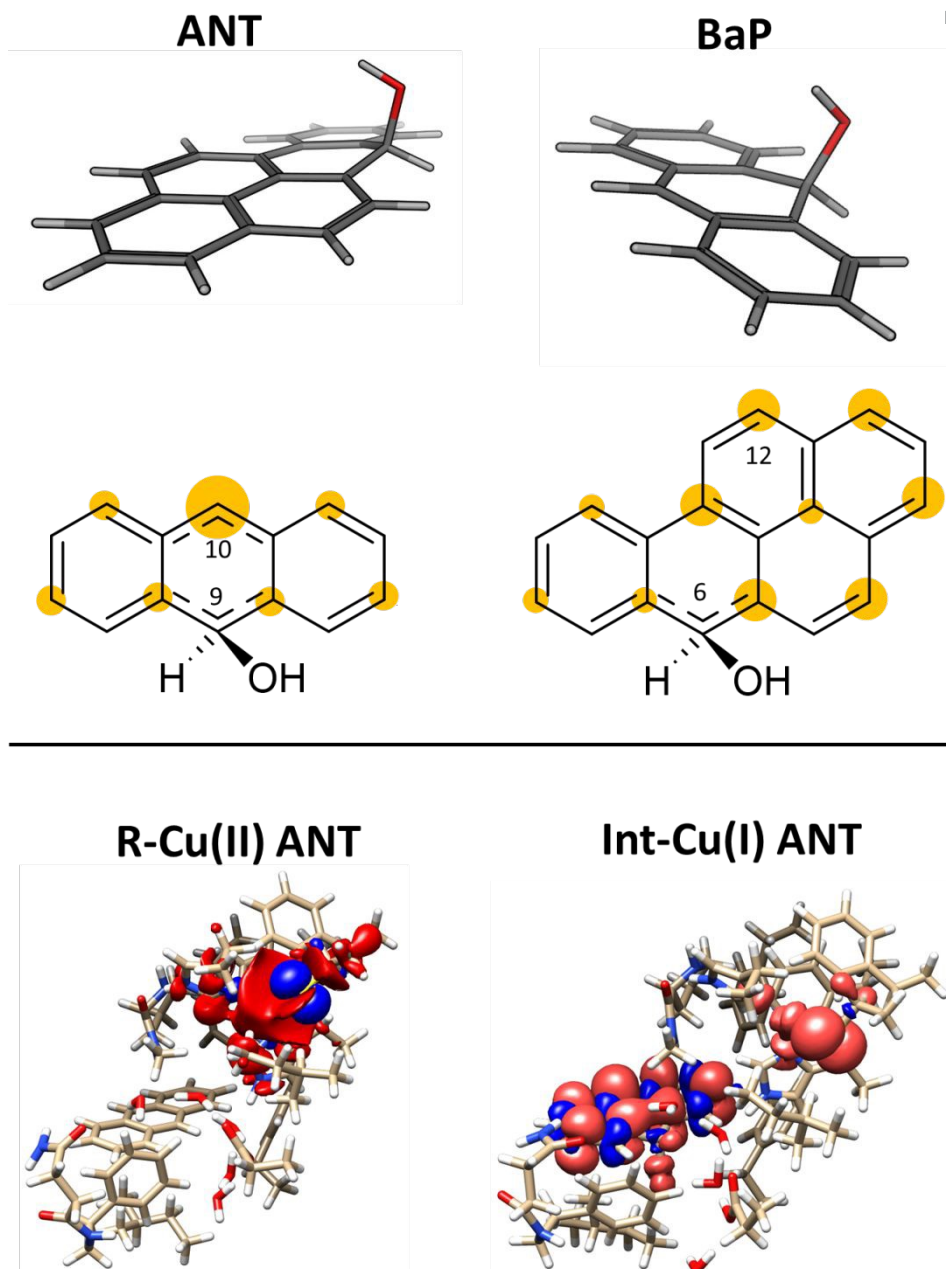
Figure 7. On the top: molecular shape and below spin populations of mono-oxidized ligand in the Int-Cu(I) intermediate for ANT and BaP. The highlighted areas in yellow on the carbon atoms are qualitatively proportional to the PBE0 spin population on that nucleus. On the bottom the total spin density for R-Cu(II) and Int-Cu(I) for ANT computed from the PBE0 level wave function at minimum geometry.
