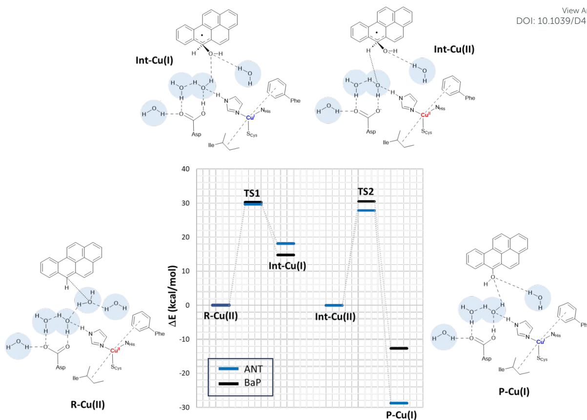
Figure 6. Proposed mechanism for the two-electron oxidation of ANT and BAP catalyzed by TvL based on DFT calculations on the extended model. Energy differences (in kcal/mol) at the PBE0-D3/TZVP/COSMO level are derived from single-point calculations on BP86-D3/TZVP/COSMO optimized structures. The structures of the various forms (reactant R-Cu(II), Cu(I)/Cu(II) intermediate Int-Cu(I) and Int-Cu(II), and product P-Cu(I)) are depicted on the side, considering BaP as example TS1 and TS2 refer to the transition states along the pathway and are associated with the first and second ET from the ligand to T1 Cu. Initially, the ligand is located in the binding pocket near T1 Cu and Asp 206 . The latter assists a proton transfer from the substrate, facilitating the ET. The proton transfer is mediated by at least one solvent molecule. The 1e oxidized form of the ligand has a tetrahedral carbon carrying an alcohol function. In the second step, T1 Cu is re-oxidized and Asp 206 deprotonated obtaining a S=0 broken-symmetry state. Then, in the second electron/proton transfer, T1 Cu is reduced and the Asp 206 side chain protonated again with the formation of a mono-hydroxy product.
