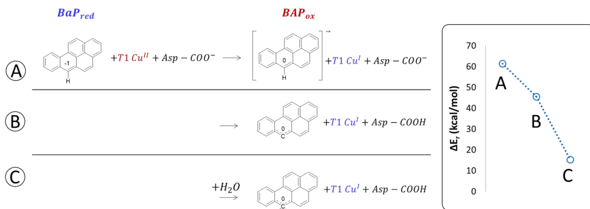
Figure 5. DFT energies (in kcal/mol) for the first oxidation of BaP, computed using the minimal model, are reported in blue. Results are based on three mechanistic hypotheses: A) mono-electronic oxidation with the formation of a carbocation, B) HAT process with the formation of a neutral radical species and protonation of Asp 206 , C) nucleophilic attack on the carbocation by a water molecule, and protonation of Asp 206 . All shown energy values are obtained from single point calculations at the PBE0-D3/TZVP/COSMO level on BP86-D3/TZVP/COSMO-optimized geometries
