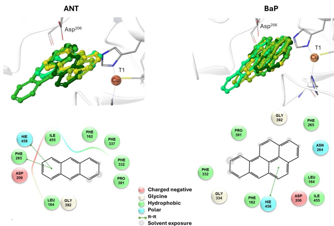
Figure 3. Top: a focus on the superimposition of the top ranked five docking poses of ANT (left) and BaP (right) to TvL (PDB: 1KYA). Bottom: interaction diagrams of the best pose obtained for each substrate to TvL.
