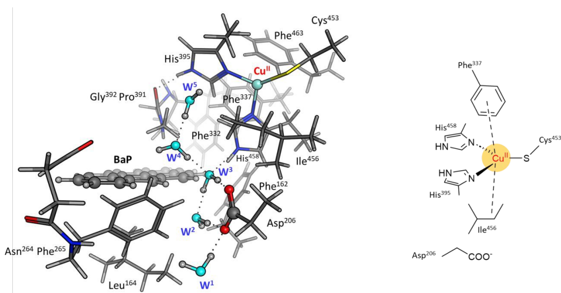
Figure 4. Right: structure of the minimal model used for our preliminary calculations, also providing details on the T1 Cu first coordination sphere. Left: structure of the extended cluster model used in this investigation. This model includes 14 residue side chains plus Cu(II), the ligand, and five water molecules (W1-5). The approach of the W4 oxygen atom to the BaP/ANT carbon atom involved in the reaction, defines the reaction coordinate for the first mono-electronic oxidation.
