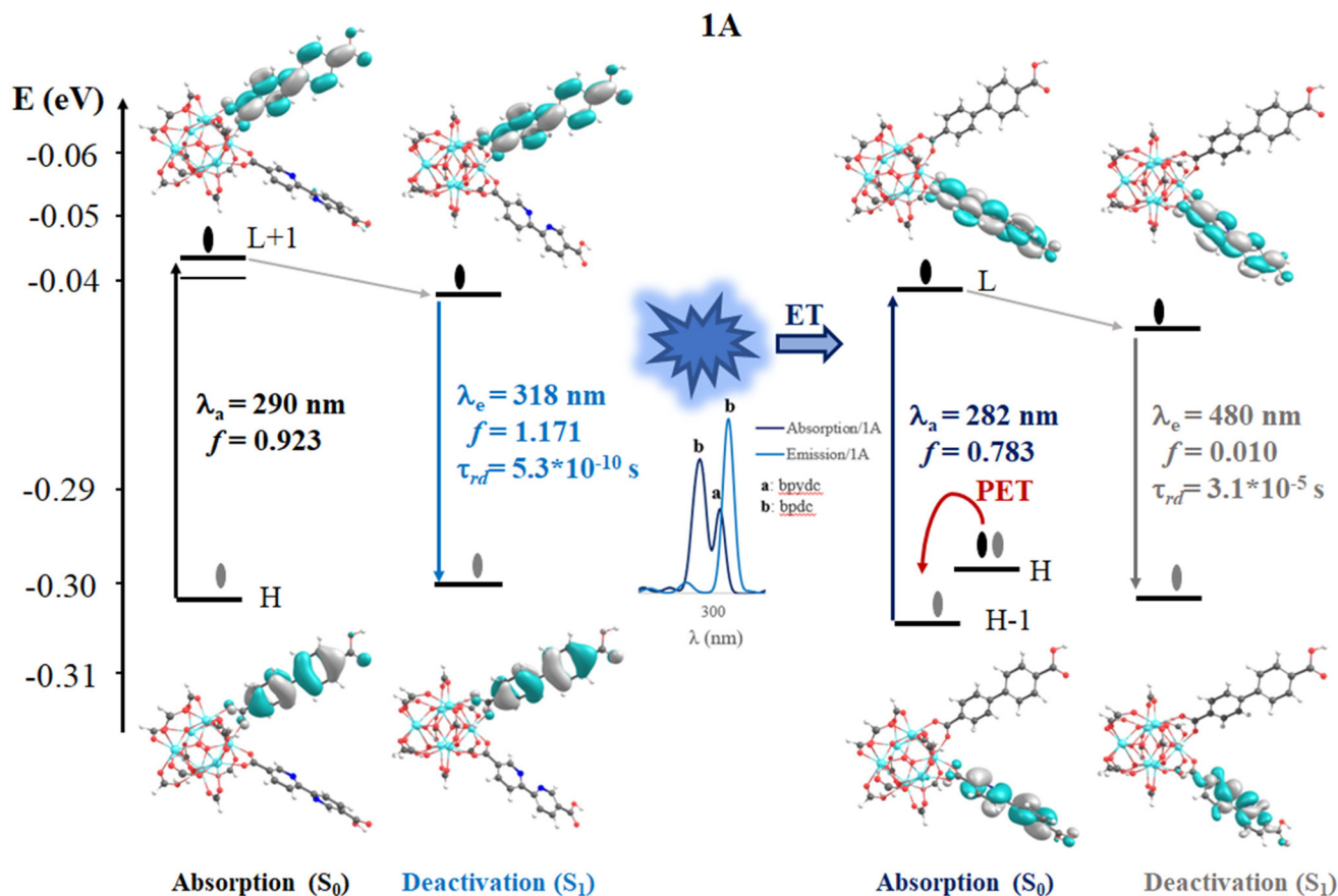
Fig. 5 Schematic representation of the photophysical mechanism based on FMOs analysis on the S 0 (absorption) and S 1 states to 1A system. Where, λ a and λ e are the computed wavelength of absorption (black and dark blue) and deactivation (light blue and gray), respectively; f is the oscillator strength; τ rad is the radiative transition lifetime and ET is energy transfer. The spectral overlap (emission bpdc /absorption at bpydc ) is represented. Isosurface contour values are set as 0.03 with TDDFT/Def2-TZPP/B3LYP theory level.
