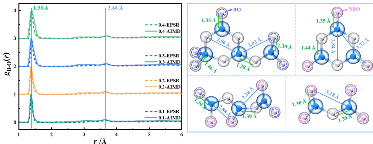
Fig. 3 Pair distribution function of B–O interactions and B–O bond lengths in different structural units in xK_2O \cdot (1-x)B_2O_3 ( 0.1 \leq x \leq 0.4 ) glass obtained by EPSR and AIMD methods.
