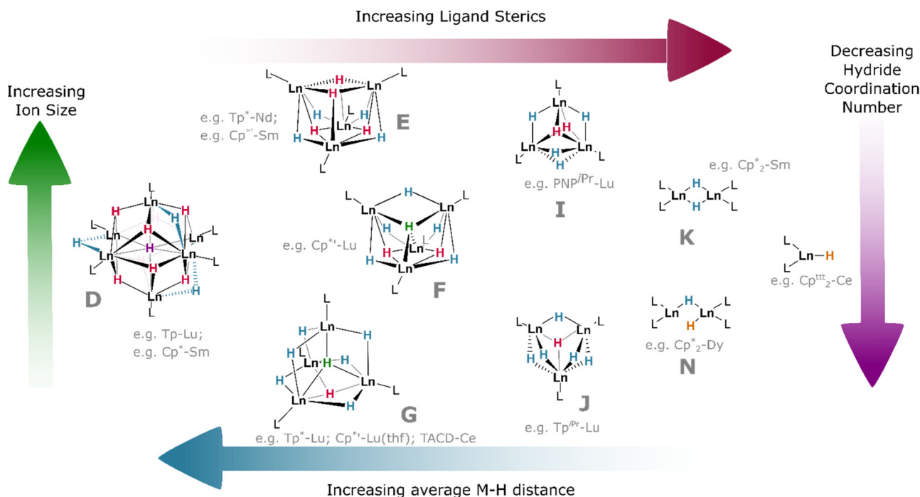
Fig. 9 Trends in structures of Ln hydride clusters with examples of L and Ln for each set. Ligand abbreviations: \text{Cp}^{\text{Lu}} = \text{C}_5(\text{CH}_3)_5 ; \text{Cp}^{\text{Sm}} = \text{C}_5(\text{CH}_3)_4(\text{SiMe}_3) ; \text{Cp}^{\text{Lu}} = \text{C}_5\text{H}_2(\text{tBu})_3 ; \text{Tp}^{\text{Lu}} = \text{tris}(3,5\text{-dimethylpyrazolyl})\text{borane} ; \text{Tp}^{\text{Lu}} = \text{tris}(3\text{-isopropyl-5-methylpyrazolyl})\text{borane} ; \text{PNP}^{\text{Lu}} = \text{N}(\text{o-C}_6\text{H}_4\text{P}(\text{tBu})_2)_2 ; TACD = \kappa^4\text{-N,N,N,N-Me}_4\text{-1,4,7,10-tetraazadodecane} .
