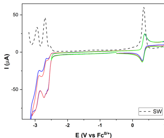
Fig. 5 CVs and SW of complex 15 in 10^{-3} M MeCN solutions containing [^nBu_4N]PF_6 10^{-1} M as the supporting electrolyte (25 °C), Pt as the counter electrode, vitreum carbon as the working electrode; potentials in V vs. Fc^+/Fc ; scan rate: 100 mV s^{-1} .
