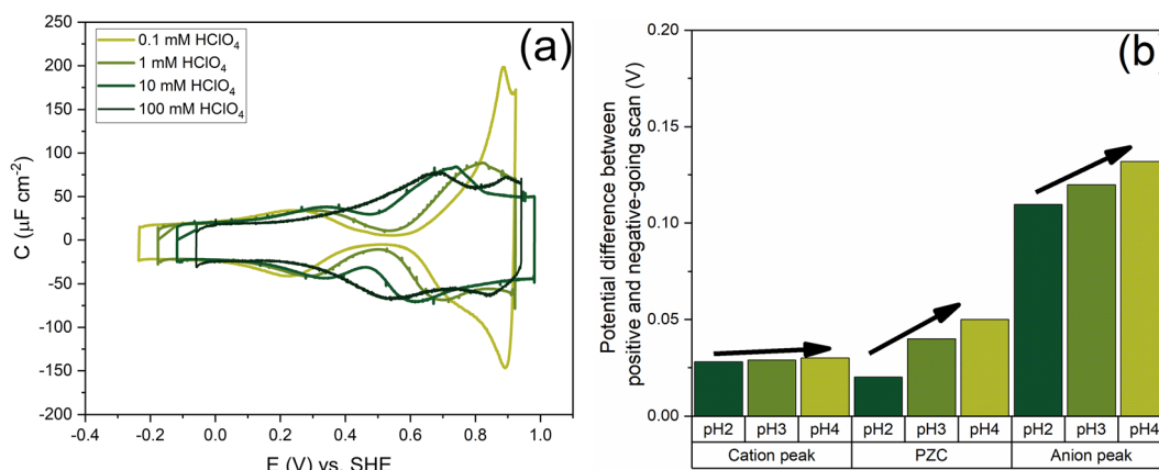
Fig. 7 Comparison of increasing HClO 4 concentration from 0.1 mM (pH 4) to 100 mM (pH 1)—(a) the voltammogram at 20 \text{mV s}^{-1} (b) the difference in the peak potential of the cation and anion-related peaks in the positive and negative-going scan and the difference in the PZC, at pH 2, pH 3 and pH 4.
