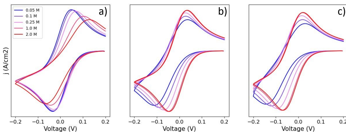
Figure 2: Simulated cyclic voltammograms for each of the pathways depicted in Scheme 2: pathways, a) 1, b) 2, and c) c. The three plots are computed using K_a^O=2 , K_a^R=10 and k_1^O=k_2^O=k_3^O=0.01 , all with a scan rate of 50 mV/s and [Q]=5\text{mM} , for [Li^+] ranging from 0.05 – 2M.
