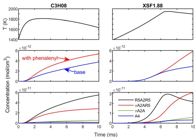
Fig. 6 Left panels: C 3 H 08 flame; right panels: XSF1.88 flame; top-row panels: flame temperature; middle-row panels: concentration of pyrene (A4) obtained with the prior mechanism 49 (designated as “base”, blue) and with the new reactions added (red); bottom-row panels: computed concentrations of pyracylene (R5A2R5, black), cyclopenta-phenalenyl ( \pi A2AR5, red), phenalenyl ( \pi A2A, green), and pyrene (A4, blue).
