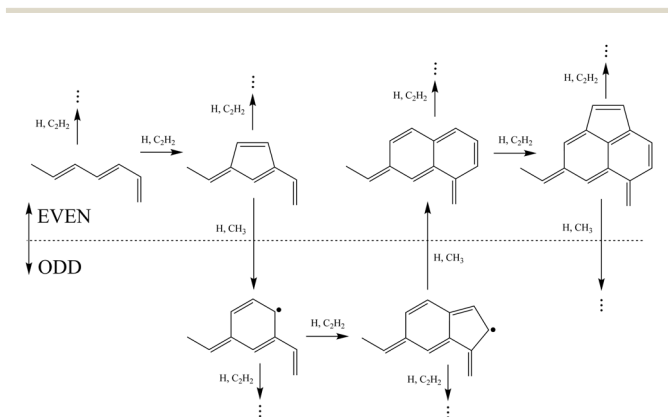
Fig. 8 PAH growth through the alternation of HAC 2H2 A and HAC H3 A reaction steps.
