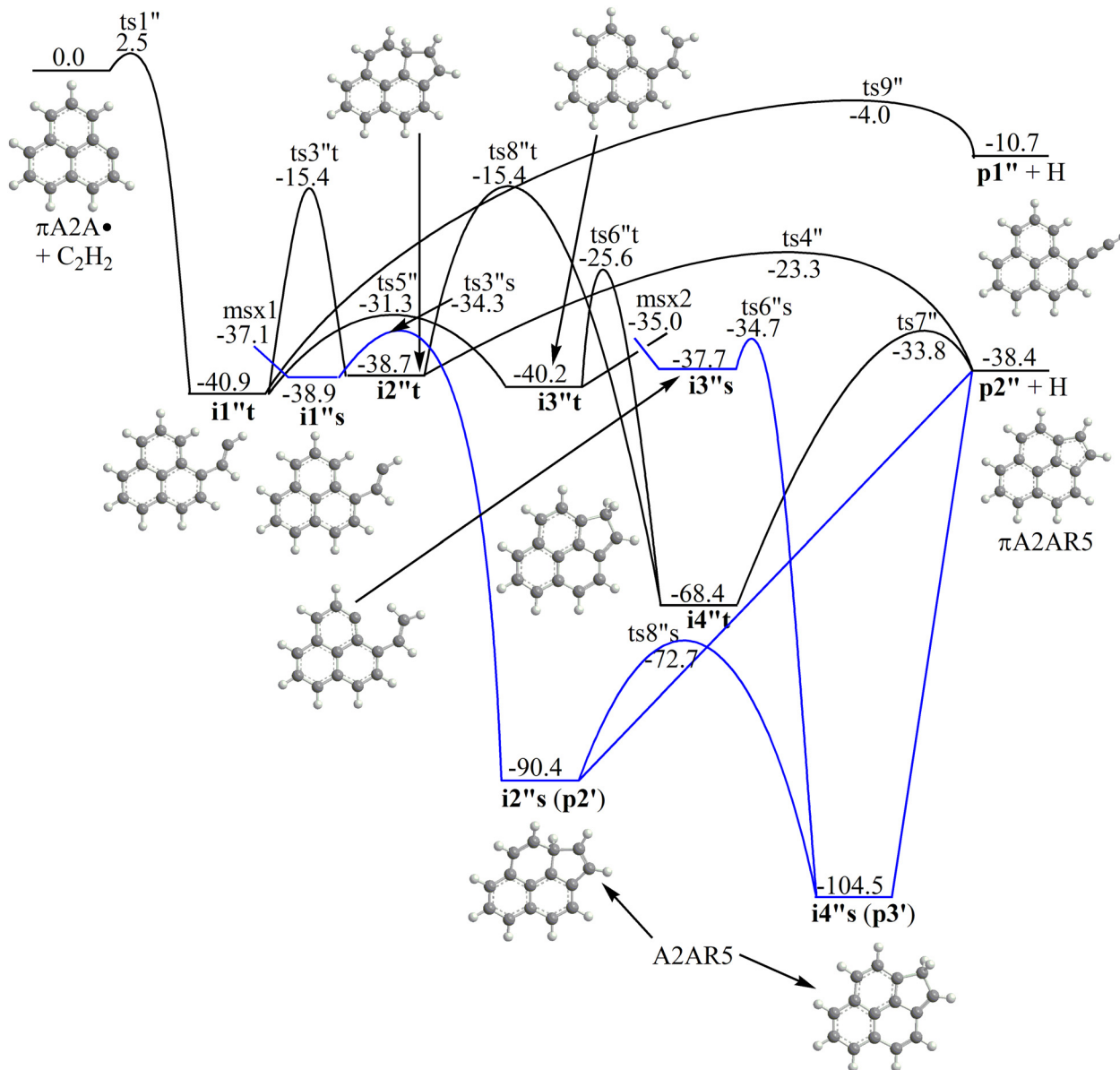
Fig. 2 Potential energy diagram for the C 13 H 8 ( \pi\text{A2A}^* ) + C 2 H 2 reaction. All relative energies given in kcal mol -1 with respect to the initial reactants are calculated at the G3(MP2,CC)//B3LYP/6-311G(d,p)+ZPE(B3LYP/6-311G(d,p)) level of theory. Black and blue curves correspond to the triplet and singlet electronic states, respectively.
