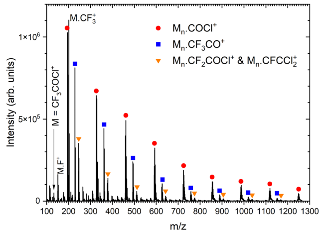
Fig. 3 The mass spectrum of (\text{CF}_3\text{COCl})_N clusters ionized at 70 eV electron energy. The clusters are produced in co-expansion of \text{CF}_3\text{COCl} molecules with Ar buffer gas at the expansion pressure of 3.8 bar.
