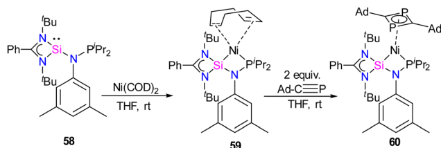
Scheme 21 (a) Synthesis of phosphine functionalized silylene–Ni(O) complex 59 . (b) The reactivity of 59 with Ad–C≡P.
