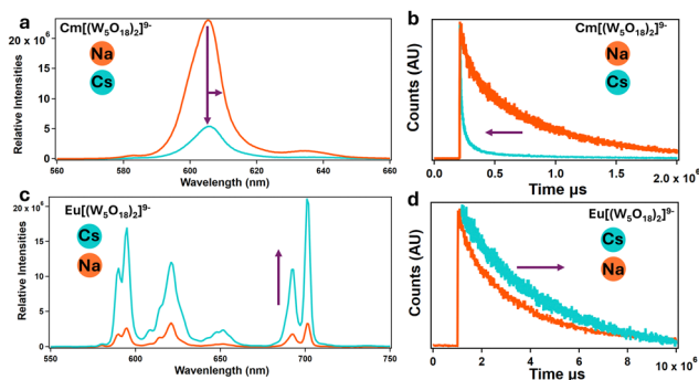
Fig. 5 Solution and time-resolved fluorescence. (a) and (b) Emission spectra of solutions of \text{CmW}_5 with sodium and cesium counterions, showing fluorescence quenching and lifetime shortening. (c) and (d) Similar experiments with \text{NdW}_5 , showing opposite behavior. Both \text{CmW}_5 and \text{EuW}_5 complexes are under 100\text{ mM} acetate buffer at a pH of 5.5 . [\text{EuW}_5] = 1\text{ mM} . [\text{CmW}_5] = 100\text{ }\mu\text{M} ( \text{Cs-CmW}_5 spectra was adjusted to compensate for the dilution for the addition of 3\text{ M} \text{CsCl} , final concentration of \text{Cs-CmW}_5 was 50\text{ }\mu\text{M} ). See Fig. S4 and S5 (ESI † ) for corresponding excitation spectra.
