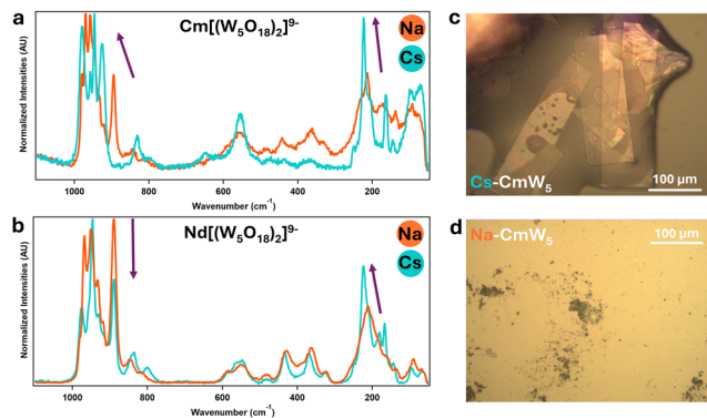
Fig. 3 Solid-state Raman microscopy of \text{CmW}_5 and \text{Nd-W}_5 (a) [\text{Cm}(\text{W}_5\text{O}_{18})_2]^{9-} with sodium (in orange) and cesium (in blue) counterions. (b) Similar experiments with [\text{Nd}(\text{W}_5\text{O}_{18})_2]^{9-} . (c) CCDC image capture of \text{Cs-CmW}_5 single crystals. This picture was taken under UV-light – the pink-orange fluorescence highlights the presence of \text{Cm}^{3+} . (d) \text{Na-CmW}_5 solution evaporated onto a microscopy slide. The material was crystalline, but the crystals were too small for XRD analysis. See Fig. S1 (ESI † ) for additional crystal pictures.
