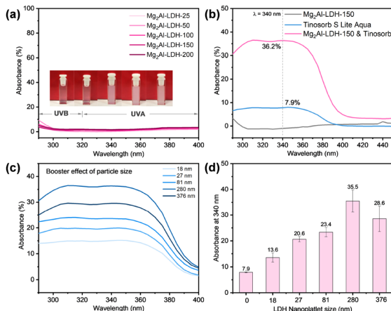
Fig. 2 (a) UV absorbance of Mg 2 Al-LDH platelet aqueous dispersions. The inset images are the dispersion of 0.1 wt% Mg 2 Al-LDH in DI water, from left to right are Mg 2 Al-LDH-25, Mg 2 Al-LDH-50, Mg 2 Al-LDH-100, Mg 2 Al-LDH-150 and Mg 2 Al-LDH-200, respectively; (b) boosting the UV absorbance of UV filter Tinosorb S Lite Aqua by Mg 2 Al-LDH-150; (c) the boosting effect of LDH platelet sizes on Tinosorb S Lite Aqua and (d) their summary of the absorbance at 340 nm. The loading of all LDHs is fixed at 0.1 wt% and Tinosorb S Lite Aqua at A 0.0003 wt%. Error bar represents the standard error from repeated experiments.
