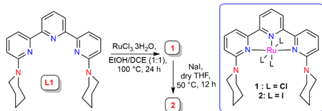
Scheme 2 Synthesis of complexes 1 and 2 .
