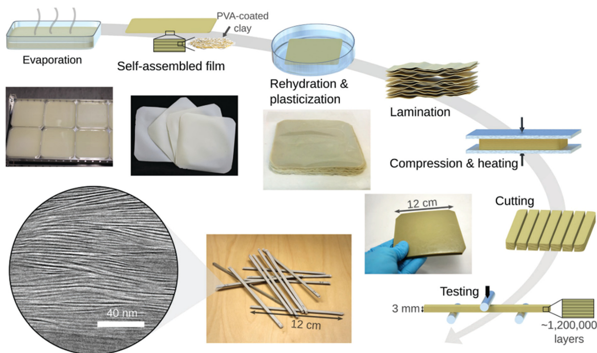
Fig. 11 The schematic of preparing the nacre-like clay/polymer composite via self-assembly technique. During evaporation, polyvinyl alcohol (PVA)-coated clay nano-platelets undergo self-assembly to form films with a thickness of approximately 60 \mu\text{m} . These films are then fused using a straightforward lamination process. The resulting plates, measuring 12 cm in width and 3–10 mm in thickness, can be cut into desired shapes for testing purposes. TEM displayed at the bottom left, exhibits the aligned bulk nanostructure with a periodicity of 2.6 nm. Reproduced from ref. 85 with permission from Wiley-VCH Verlag GmbH & Co. KGaA, Weinheim, copyright 2017.
