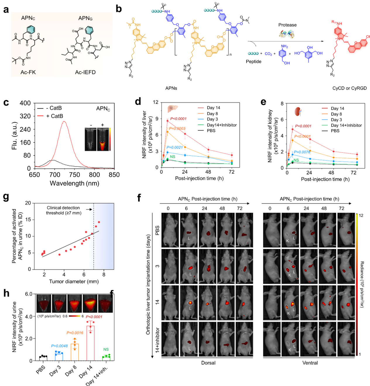
Fig. 2 NIRF imaging and urinalysis of APN c for early cancer diagnosis. (a). Chemical structures of protease-responsive peptide brushes (Ac-FK and Ac-IEFD) for APN 5 design. (b). Chemical structures of APN 5 and the corresponding fluorogenic fragments in response to the respective proteases (CyCD or CyRGD). ( R_1 = \text{H} or (\text{CH}_3)_2\text{NCO} , R_2 = \text{HP}\beta\text{CD} or cRGD, R_3 = \text{H} or \text{CH}_2\text{CHOHCH}_3 ). (c). NIR-fluorescence spectra of APN c ( 10 \mu\text{M} ) in the absence or presence of Cat B ( 0.5 \mu\text{g} ) in a PBS solution at 37^\circ\text{C} . (d and e). NIRF intensity versus time curves of the liver (d) and kidney (e) after injection of APN c in live mice ( n = 4 ). (f). NIRF imaging of live mice with implanted tumours after APN c injection at different time points (0, 3, and 14 d). White circles display the tumour (T), liver (L), and kidney (K). (g). The correlation between the percentage of activated APN c in urine and tumour size was studied by linear regression analysis. (h). APN c was injected at different time points and the fluorescence intensity of the activated probe was collected in urine from each group of mice ( n = 4 ). PBS versus tumour-implantation groups. Reproduced with permission from ref. 33. Copyright 2022, Springer Nature.
